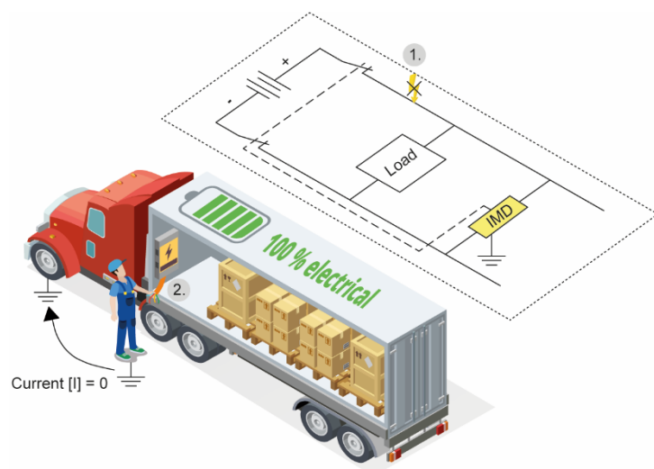
Figure 6: Electrical outlets from Bucher Hydraulics are fitted with high-impedance Insulation Monitoring Devices and thus ensure a fully safe energy supply in commercial vehicles.
