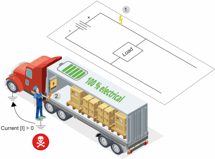
Figure 4: Contact with an open line (secondary fault) has high risk potential in the event of an insulation fault (primary fault) in insulated grids.
