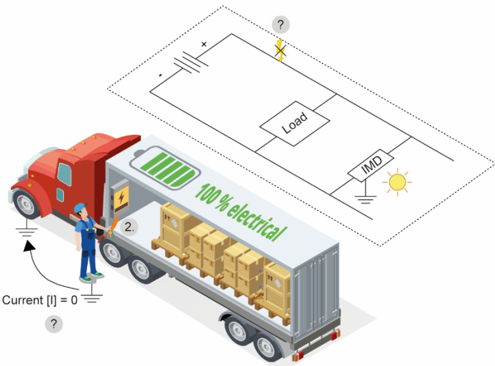
Figure 5: Insulation faults in commercial vehicles are reliably detected by "Insulation Monitoring Devices" (IMDs). This component ensures improved safety in electric vehicles.
